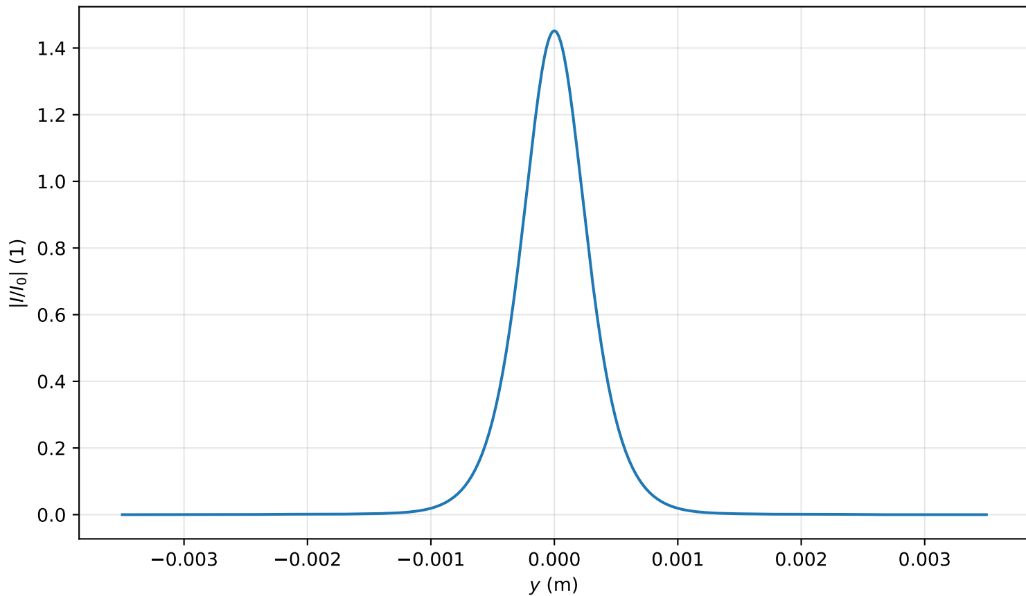
Intensity profile I(x=0, y, z=3.742)/I_0 , P_{in}=0.9P_{cr} , artificial time
